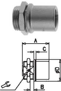
ED : Front mount, protruding
