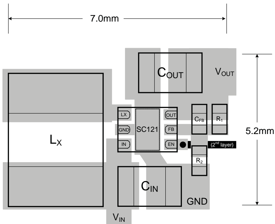
Figure 4 — Layout Drawing
