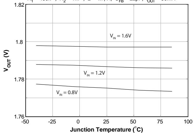
Temperature Reg. — High Load ( V_{OUT} = 1.8V )
