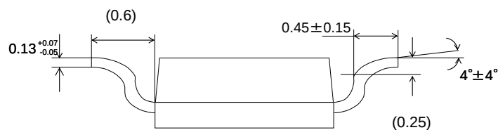
END VIEW
