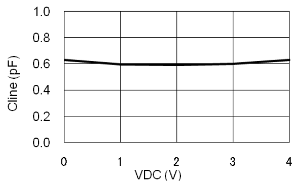
Voltage – Capacitance Characteristic
