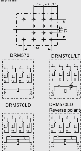
Circuit diagram PIN top view Dimensions are in mm
