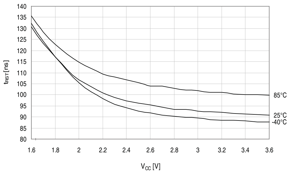
Figure 34-318. Minimum Reset pin pulse width vs. V CC .
