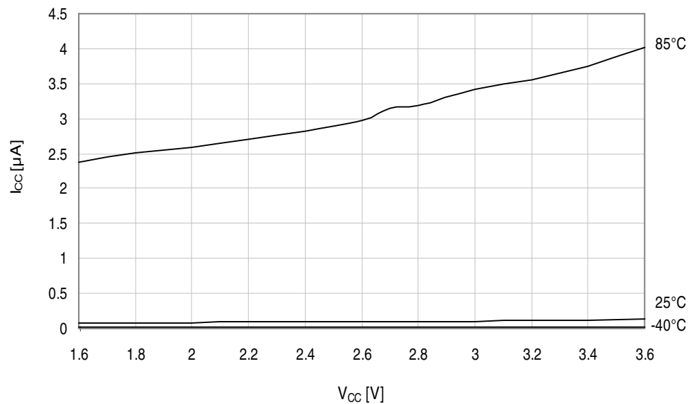
Figure 34-286. Power-down mode supply current vs. V_{CC} .
