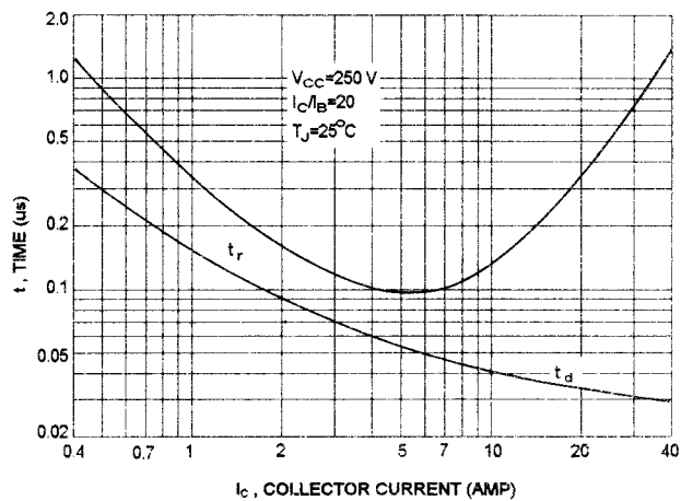
TURN-ON TIME
