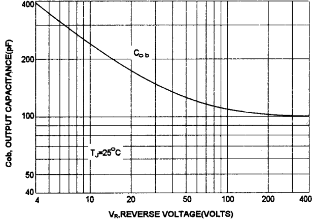
OUTPUT CAPACITANCES
