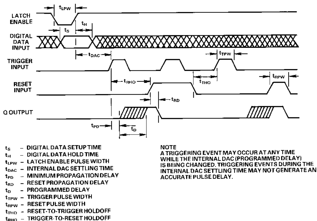
Figure 1. System Timing Diagram
