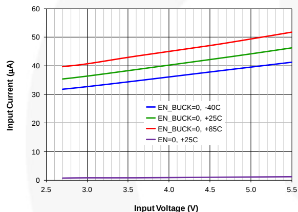
Figure 21. Shutdown Current vs. Input Voltage and Temperature
