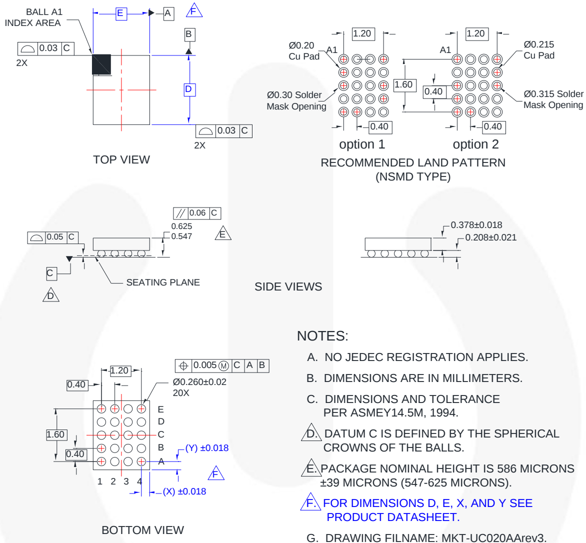
Figure 41. 20-Ball, Wafer-Level Chip-Scale Package (WLCSP), 4x5 Array, 0.4 mm Pitch, 250 \mu m Ball
