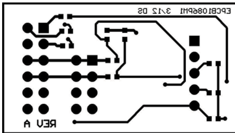
Figure 6. DS1086LPMB11 Peripheral Module PCB Layout—Solder Side
