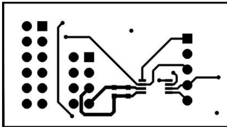
Figure 3. DS1086LPMB1 Peripheral Module PCB Layout—Component Side
