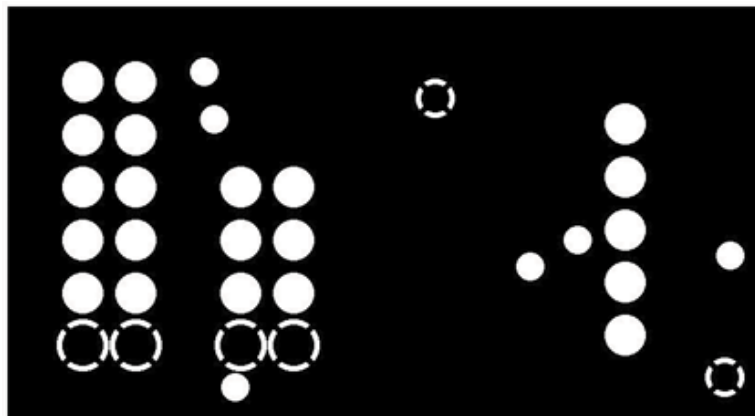
Figure 4. DS1086LPMB1 Peripheral Module PCB Layout—Inner Layer 1 (Ground)
