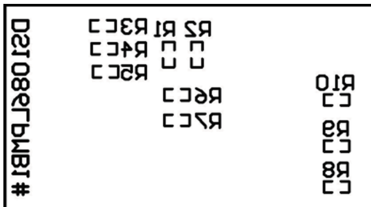
Figure 7. DS1086LPMB11 Peripheral Module Component Placement Guide—Solder Side
