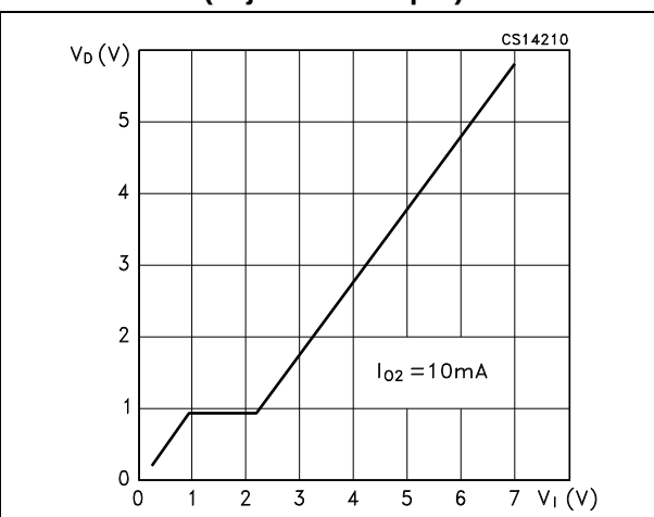
Figure 10. Dropout voltage vs. input voltage (adjustable output)
