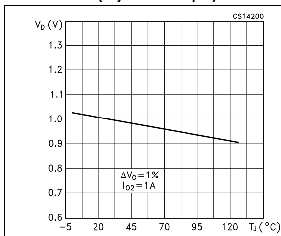
Figure 9. Dropout voltage vs. temperature (adjustable output)
