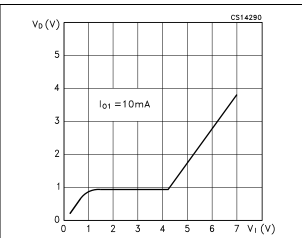
Figure 18. Dropout voltage vs. input voltage
