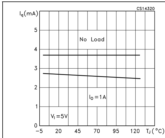
Figure 21. Quiescent current vs. temperature (fixed/adj. version)
