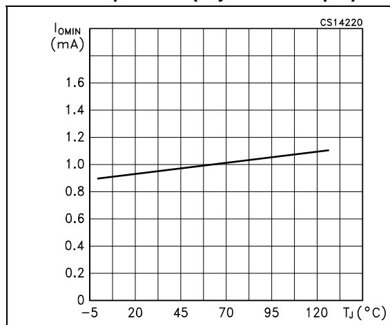
Figure 11. Minimum load current vs. temperature (adjustable output)
