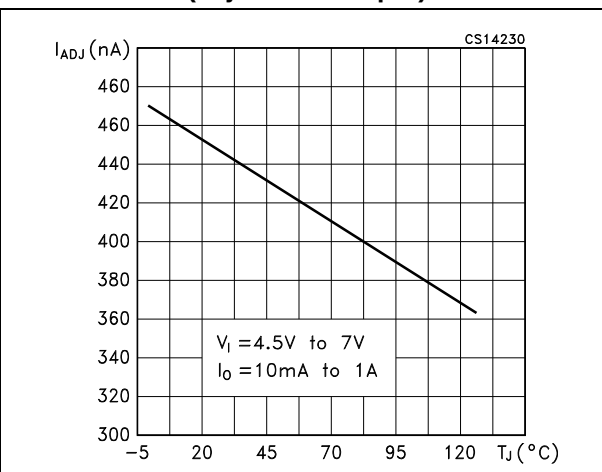
Figure 12. Adjust pin current vs. temperature (adjustable output)
