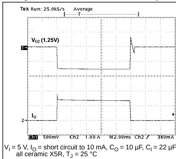
Figure 23. Short-circuit removal response
