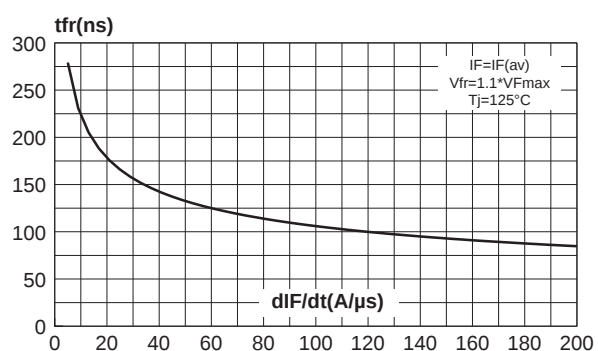
Fig. 16: Forward recovery time versus dI_F/dt (90% confidence).
