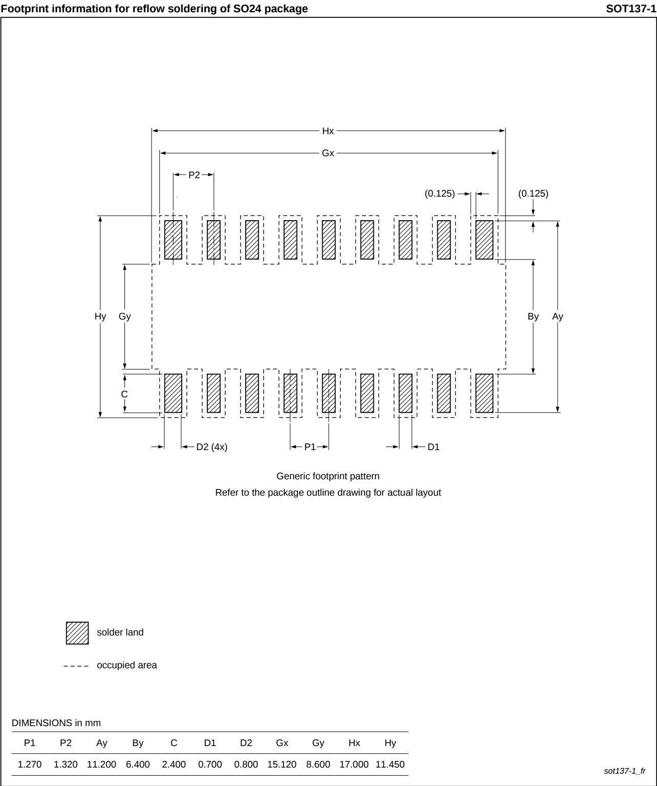
Fig 31. PCB footprint for SOT137-1 (SO24); reflow soldering
