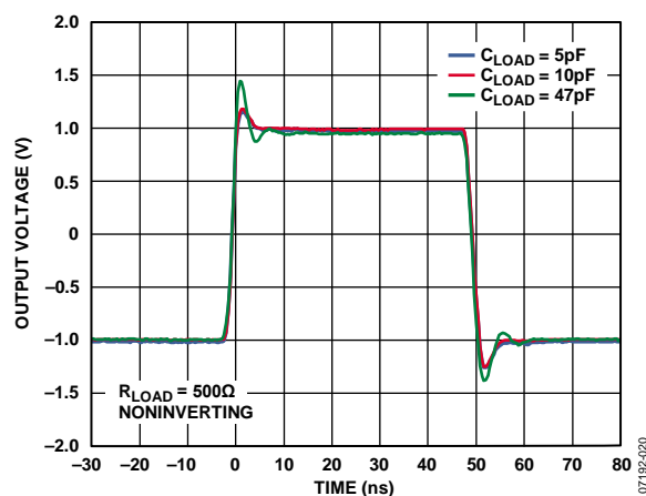
Figure 20. Large-Signal Pulse Response of the High Current Driver for Various Values of Load Capacitance, C_{LOAD} , and R_{LOAD} = 500\ \Omega —See Figure 56
