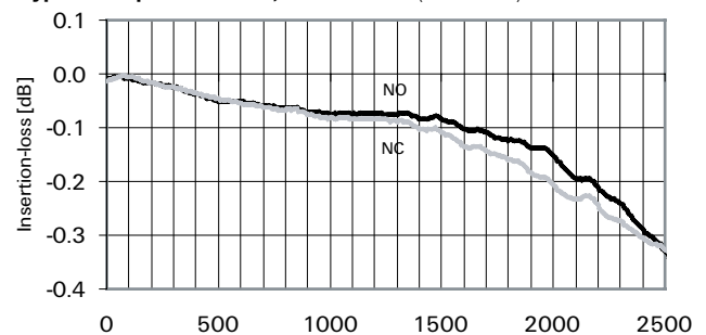
Typical RF performance, 75 \Omega version (continued)
