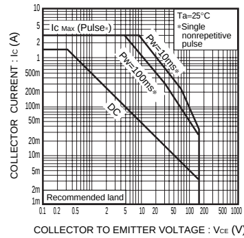
Fig.9 Safe operating area (2SD2211)
