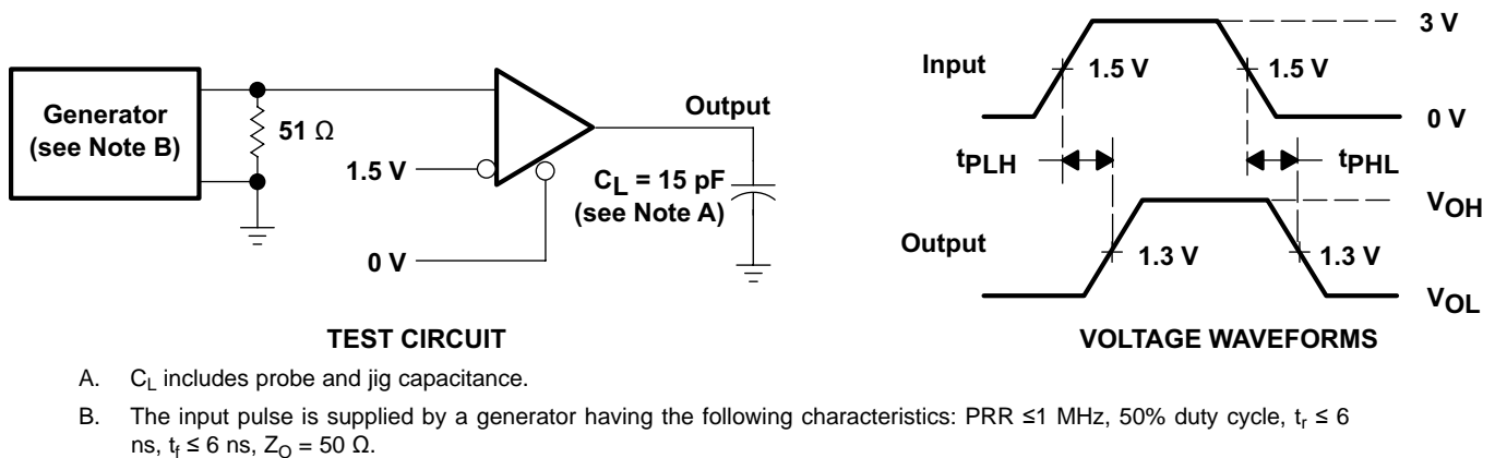
Figure 6. Receiver Test Circuit and Voltage Waveforms
