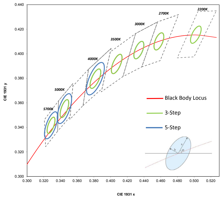
Figure 7. 3-step and 5-step MacAdam ellipse color bins.
