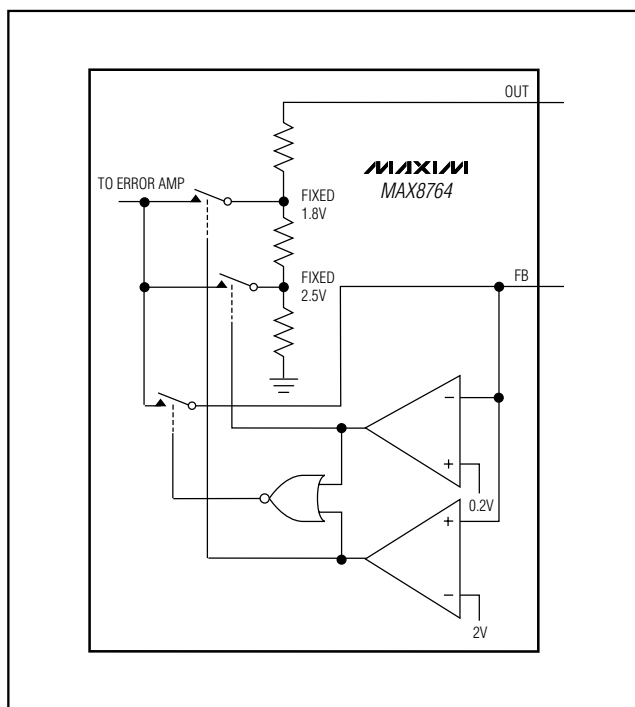
Figure 6. Feedback Mux
