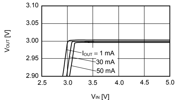
S-1323B30 ( T_a = 25^\circ\text{C} )
