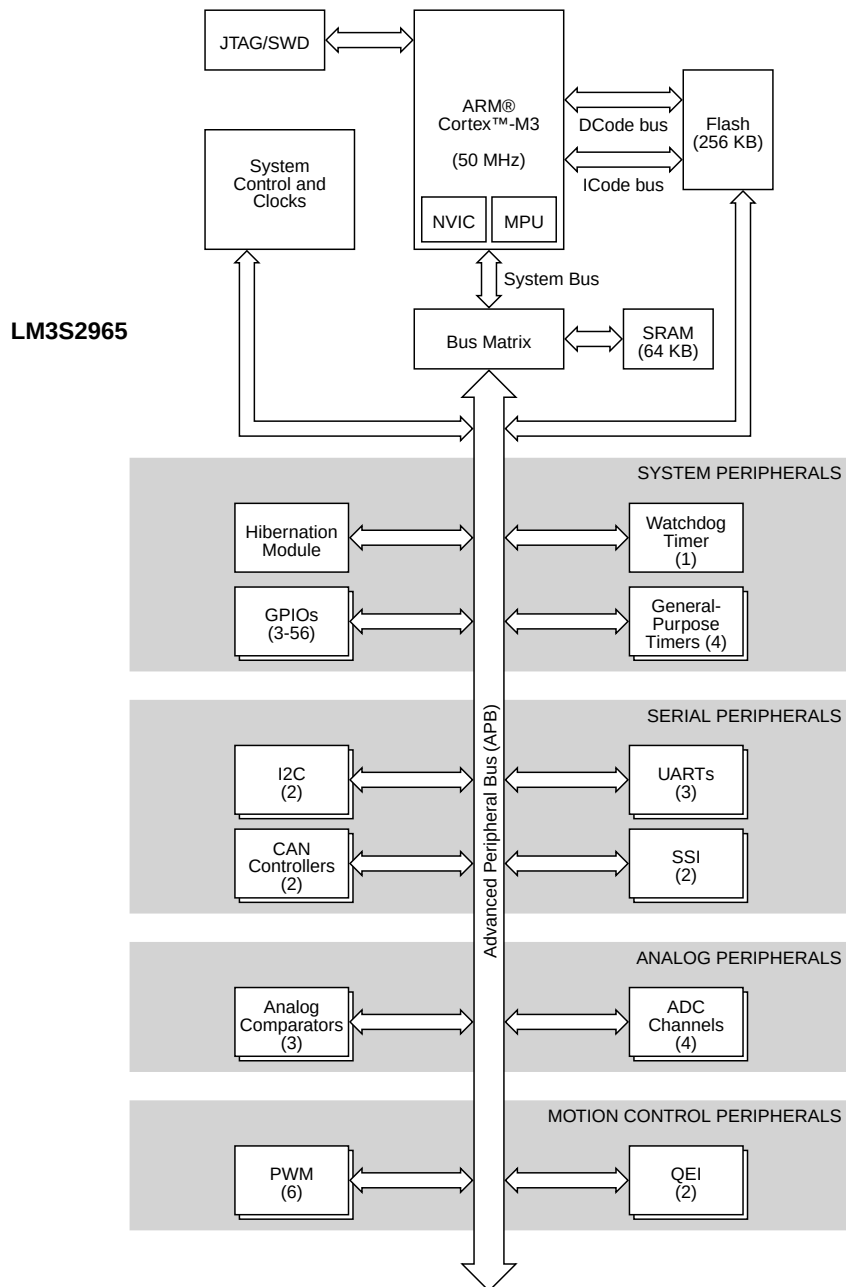
Figure 1-1. Stellaris® LM3S2965 Microcontroller High-Level Block Diagram
