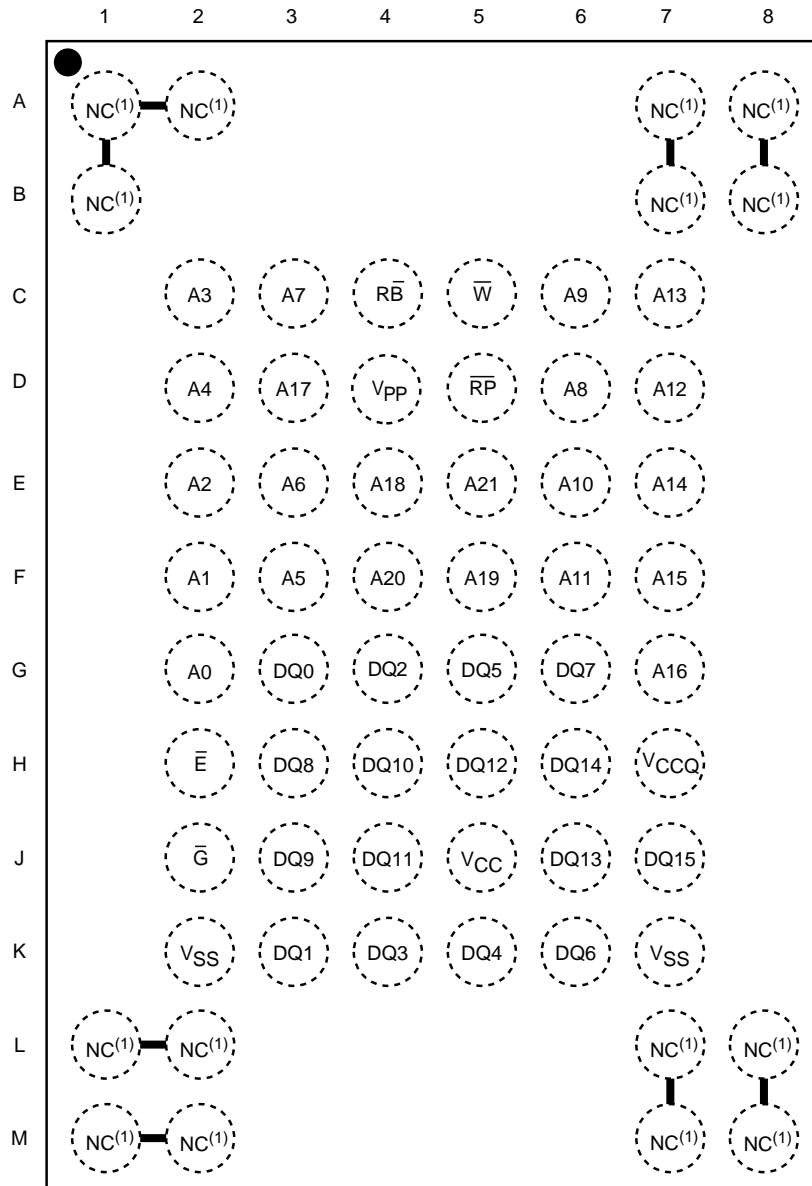
Figure 4. TFGBA Connections (Top view through package)
