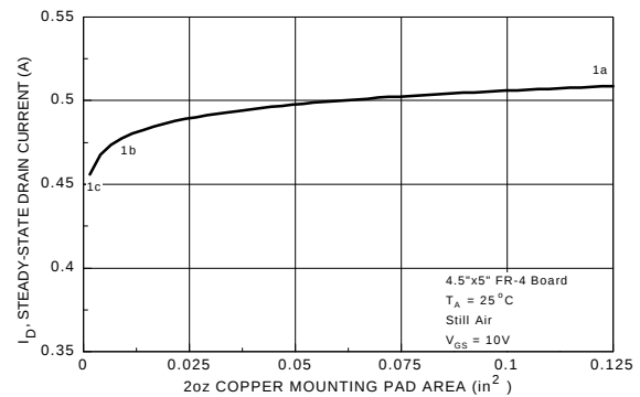
Figure 24. N-Ch Maximum Steady-State Drain Current versus Copper Mounting Pad Area.
