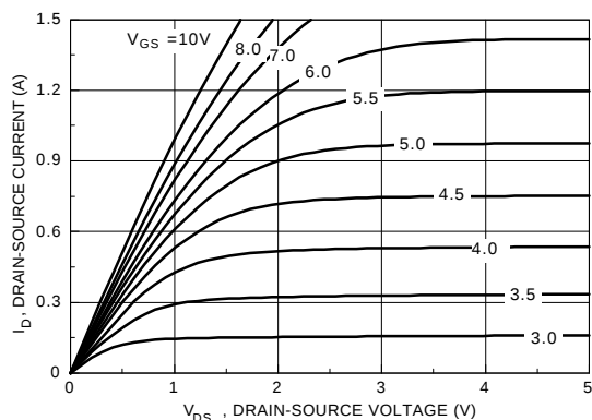
Figure 1. N-Channel On-Region Characteristics.
