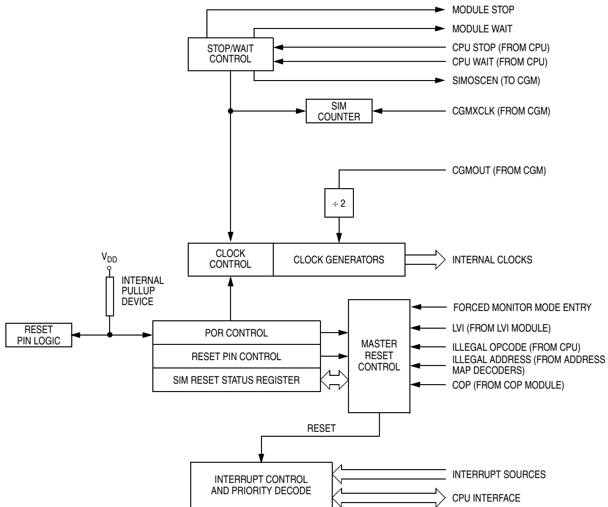
Figure 16-1. SIM Block Diagram
