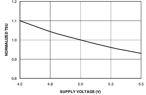
NORMALIZED TSU VS. SUPPLY VOLTAGE ( T_A = 25^\circ C )
