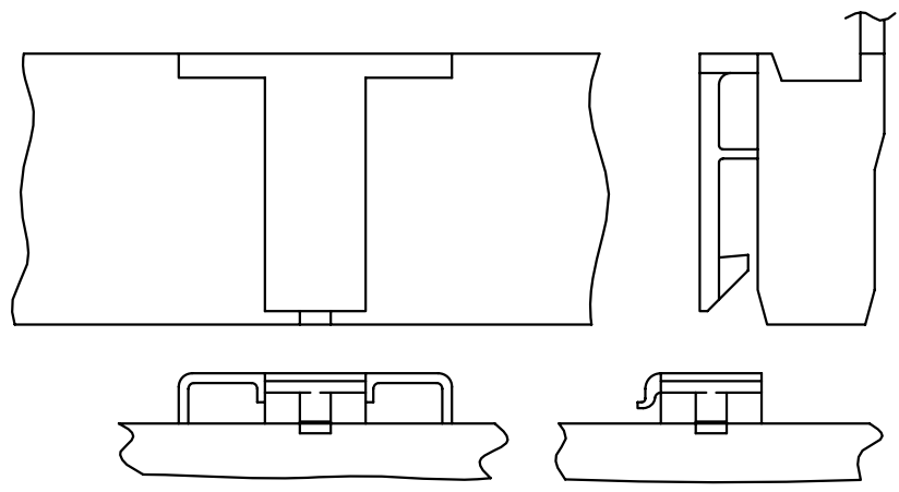
VIEW Z LATCH STYLE 2
