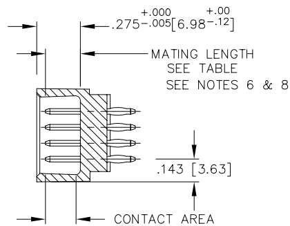
SECTION X-X
