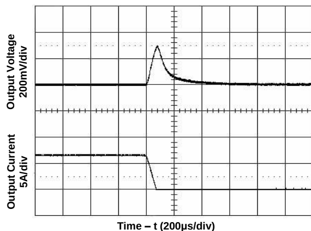
Figure 7. Transient Load Response
