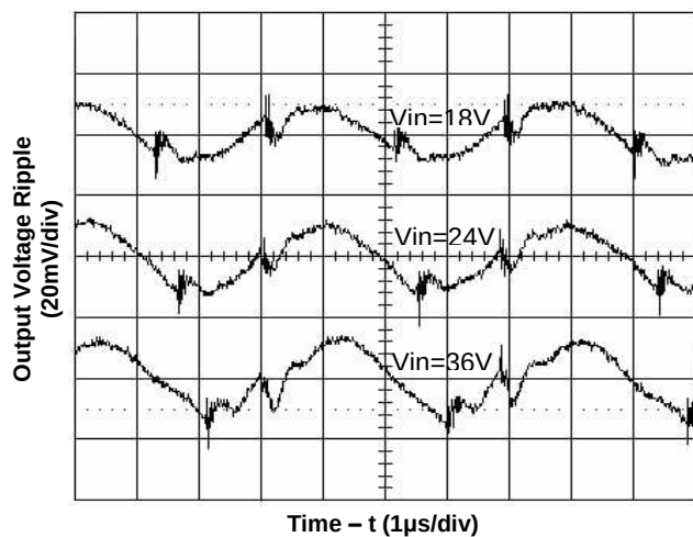
Figure 5. Output Ripple Voltage at Full Load
