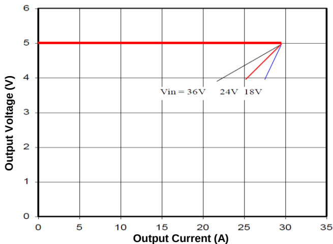
Figure 10. Output Characteristics
