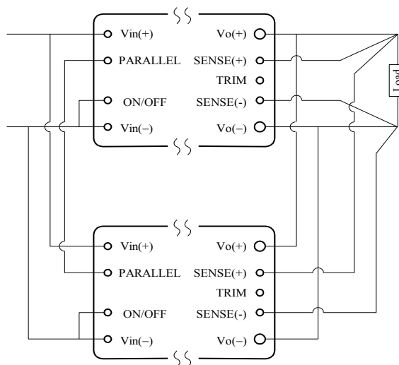
Fig. 20 Circuit Configuration for Active Current Share
