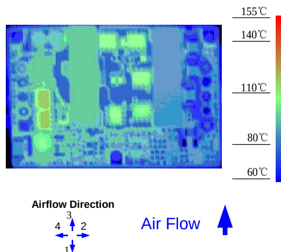
Figure 12. Thermal Image for Airflow Direction 3 (24.1A output, 65°C ambient, 200 LFM, typical Vin, open frame unit using soldering interface)
