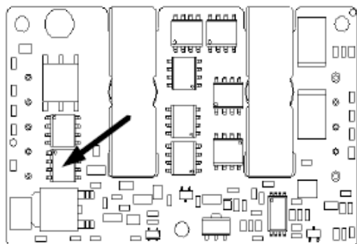
Figure 21. Temperature Monitoring Location
