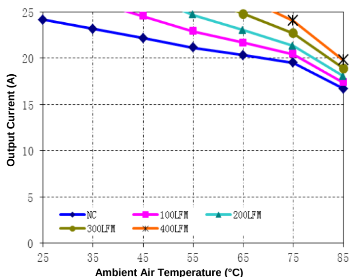
Figure 13. Current Derating Curve for Airflow Direction 4 (Ref. Fig. 14 for Airflow Direction; Vin = 24V open frame unit using socket interface)
