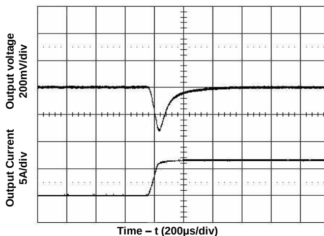
Figure 8. Transient Load Response
