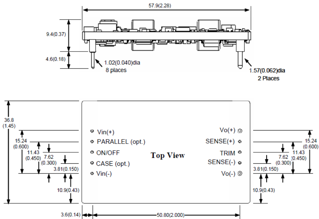
Figure 22. Open frame converter
