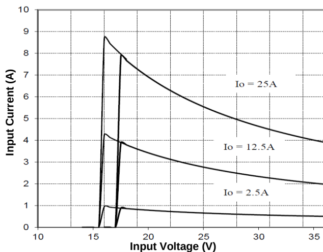
Figure 9. Input Characteristics
