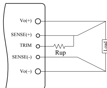
Figure 19. Circuit to Increase Output Voltage
