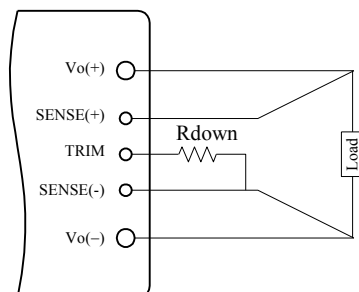
Figure 18. Circuit to Decrease Output Voltage
