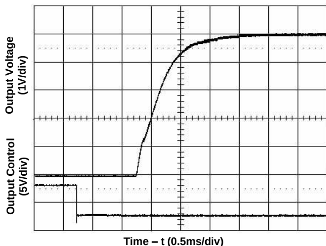
Figure 3. Start-Up from Enable Control Input voltage 24V, Output current 25A
