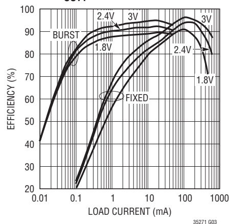
Efficiency vs Load Current and V_{IN} for V_{OUT1} = 3.3\text{V} at 1.2MHz
