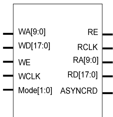
FIGURE 2. QuickRAM Module
