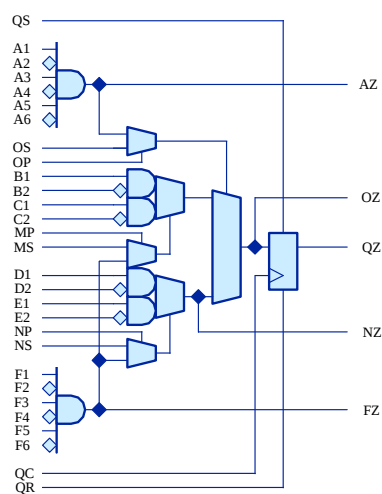
FIGURE 4. Logic Cell
