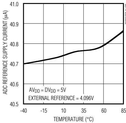
ADC REFERENCE SUPPLY CURRENT vs. TEMPERATURE
