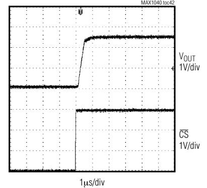
DYNAMIC RESPONSE RISE TIME ( R_{LOAD} = 10k\Omega , C_{LOAD} = 100pF )
