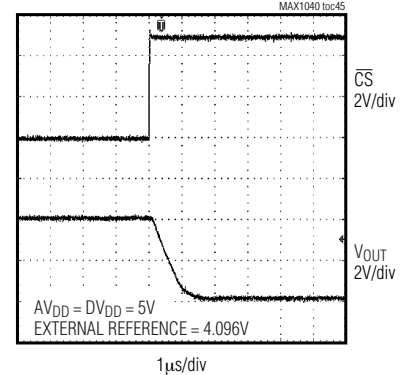
DYNAMIC RESPONSE FALL TIME ( R_{LOAD} = 10k\Omega , C_{LOAD} = 100pF )
