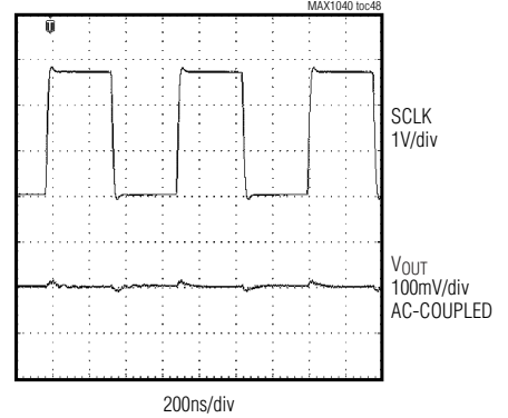
DAC DIGITAL FEEDTHROUGH ( R_{LOAD} = 10k\Omega , C_{LOAD} = 100pF , CS = HIGH, DIN = LOW)
