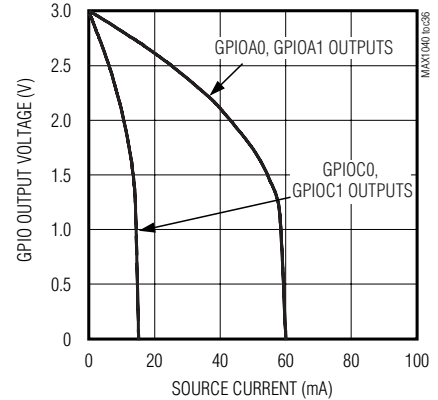
GPIO OUTPUT VOLTAGE vs. SOURCE CURRENT
