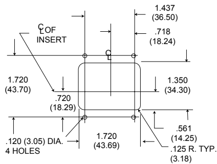
-33 Front Mount
