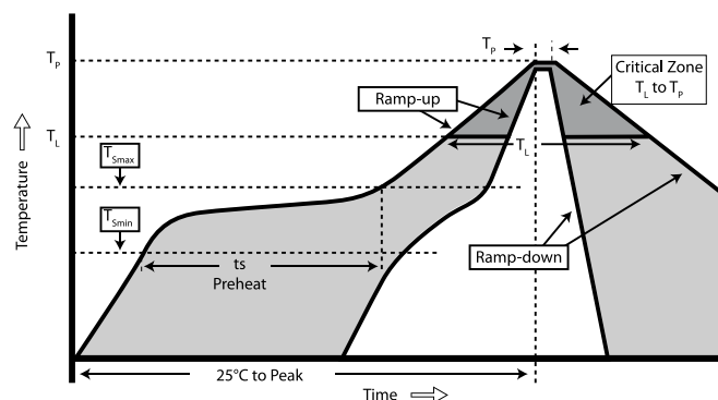
Figure 4. Soldering profiles
