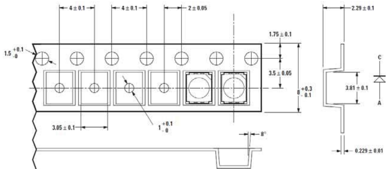
Figure 10. Tape Dimensions
