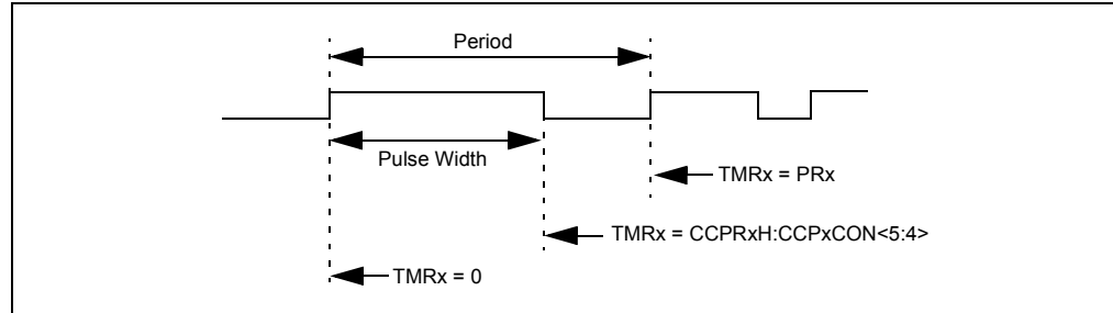
FIGURE 3-8: PWM ANALYSIS
