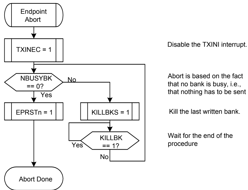
Figure 27-18. Abort Algorithm
