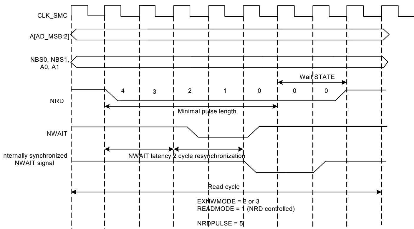
Figure 15-29. NWAIT Latency
