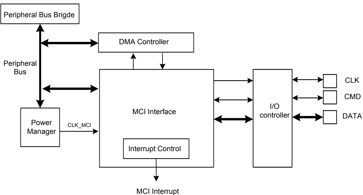
Figure 31-1. MCI Block Diagram
