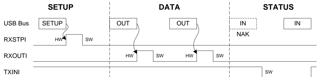
Figure 27-14. Control Write
