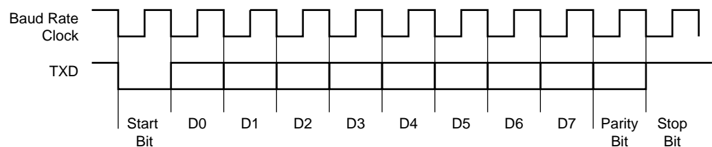
Figure 25-2. Character Transmit
