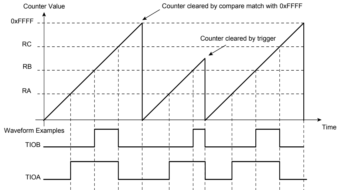
Figure 28-7. WAVSEL= 0 With Trigger
