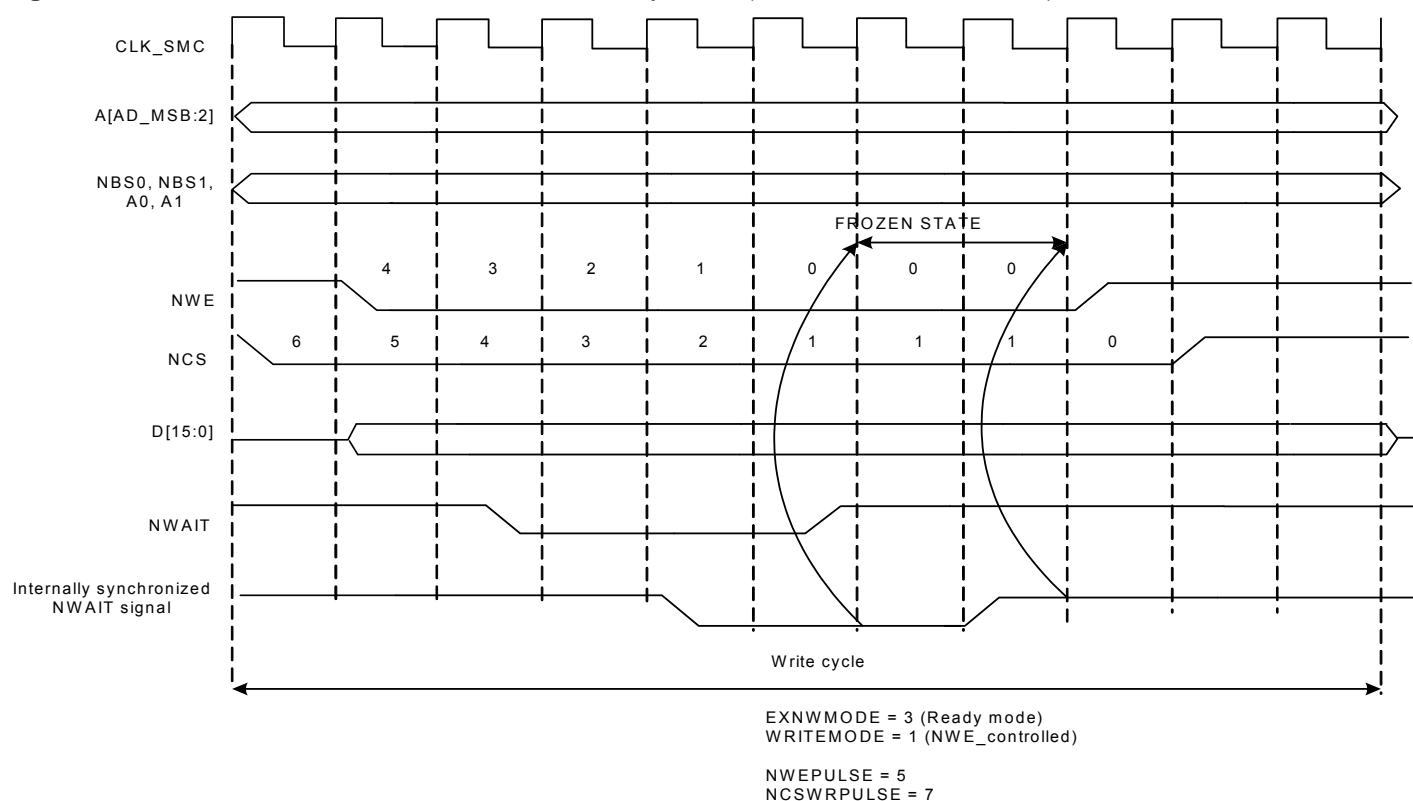
Figure 15-27. NWAIT Assertion in Write Access: Ready Mode ( \text{MODE.EXNWMODE} = 3 ).
