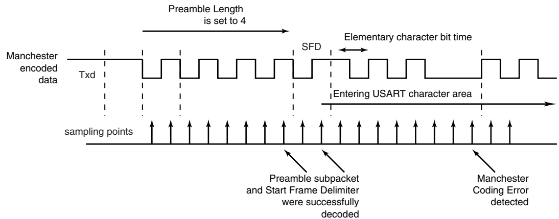
Figure 25-50. Manchester Error
