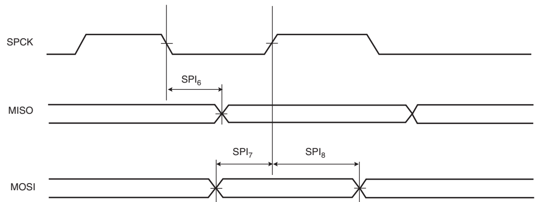
Figure 36-13. SPI Slave mode with (CPOL= 0 and NCPHA= 1) or (CPOL= 1 and NCPHA= 0)
