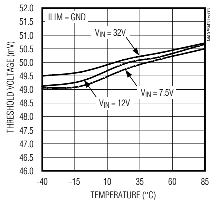
CURRENT-LIMIT/CIRCUIT-BREAKER THRESHOLD VOLTAGE vs. TEMPERATURE
