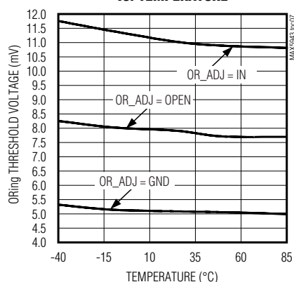
ORing THRESHOLD VOLTAGE vs. TEMPERATURE
