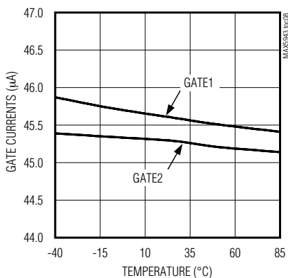
GATE CURRENTS vs. TEMPERATURE
