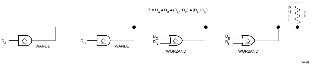
Figure 21: Open-Drain Buffers Implement a Wired-AND Function
