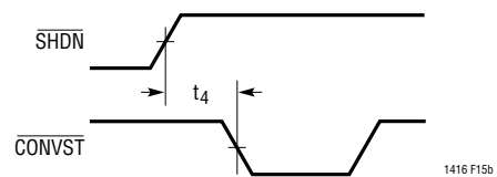
Figure 15b. \overline{\text{SHDN}} to \overline{\text{CONVST}} Wake-Up Timing
