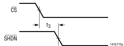
Figure 15a. \overline{\text{CS}} to \overline{\text{SHDN}} Timing
