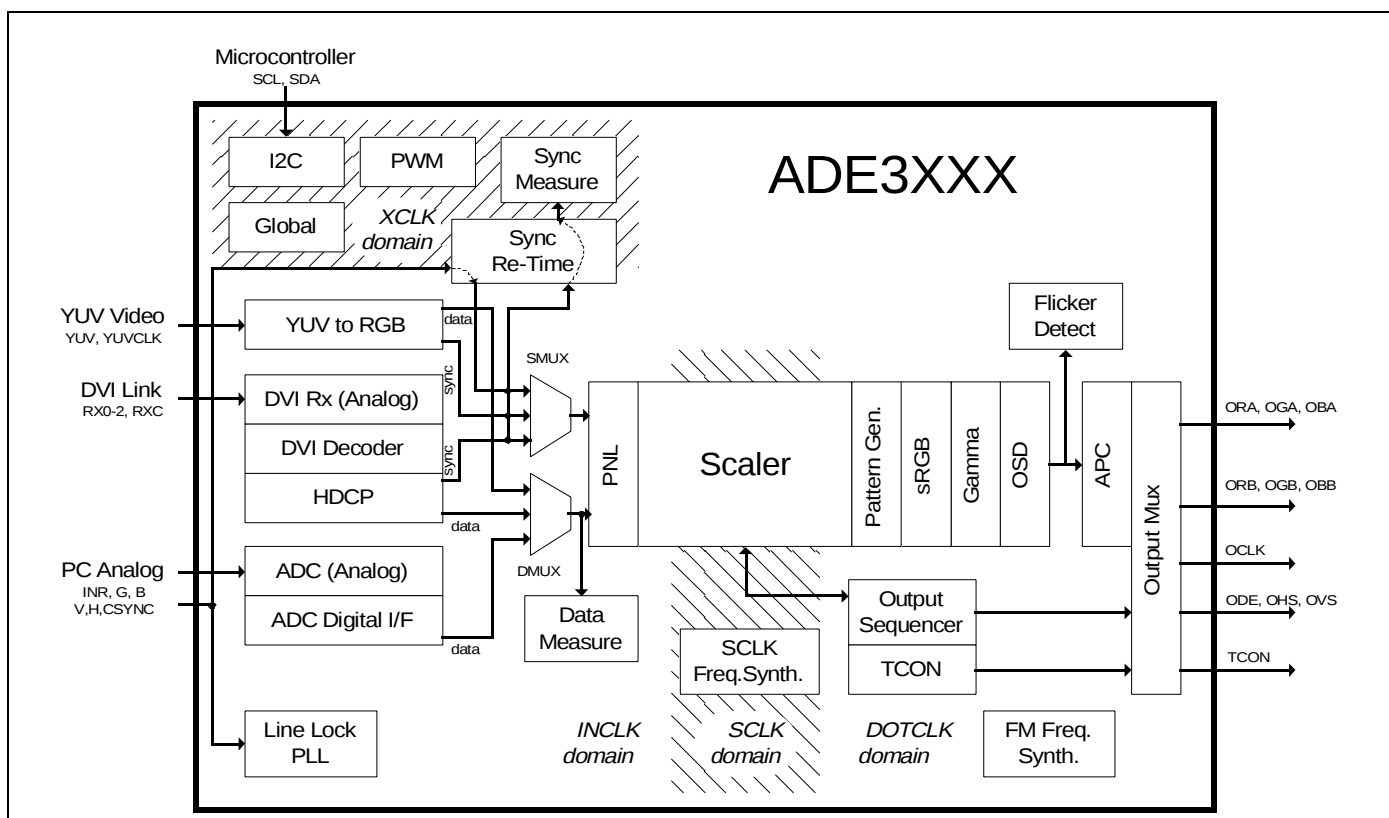
Figure 2: Clock Domains
