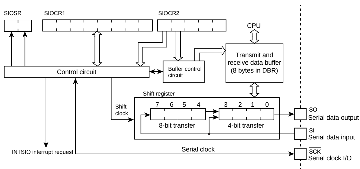
Figure 10-1 Serial Interface
