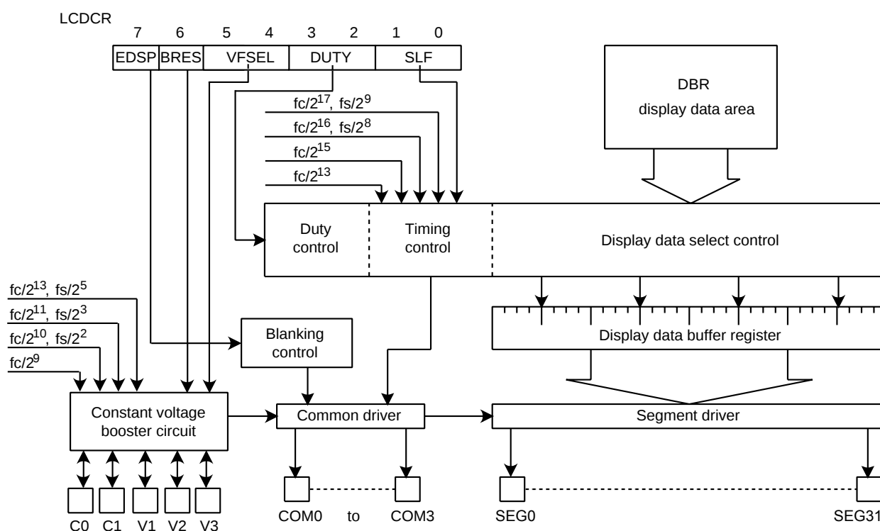
Figure 13-1 LCD Driver
