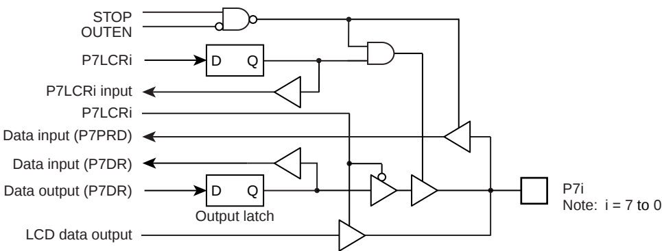
Figure 5-7 Port 7
