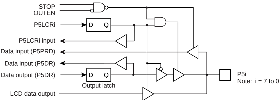
Figure 5-5 Port 5
