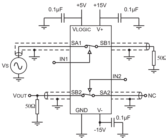
Figure 7 - Channel-to-Channel Crosstalk
