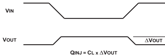
Figure 5. Charge Injection
