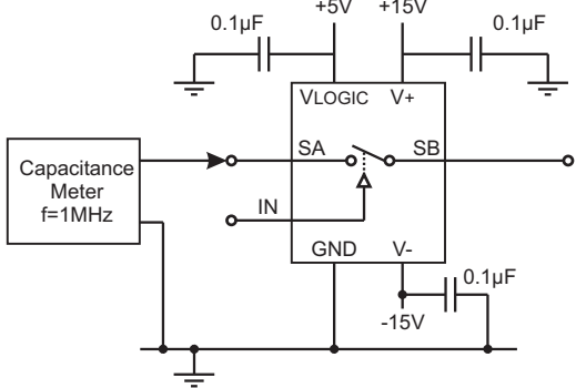
Figure 8 - Off Capacitance
