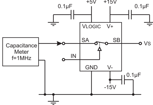
Figure 9 - On Capacitance
