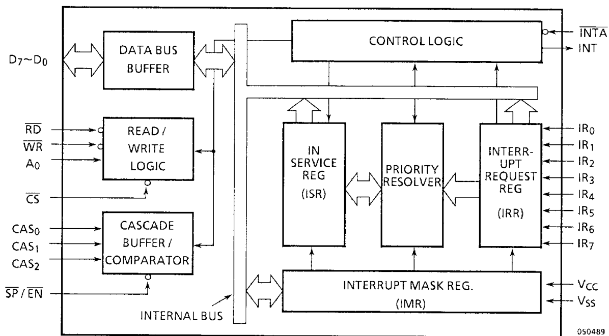
Figure 4.1 BLOCK DIAGRAM
