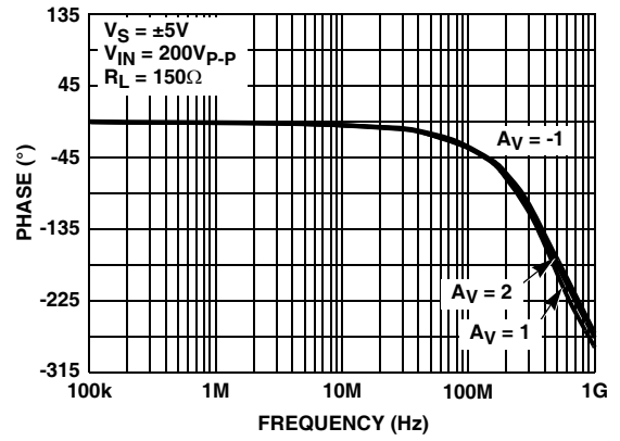
FIGURE 2. PHASE RESPONSE
