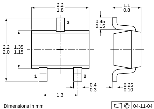
Fig 15. Package outline PDTC124EU (SOT323/SC-70)
