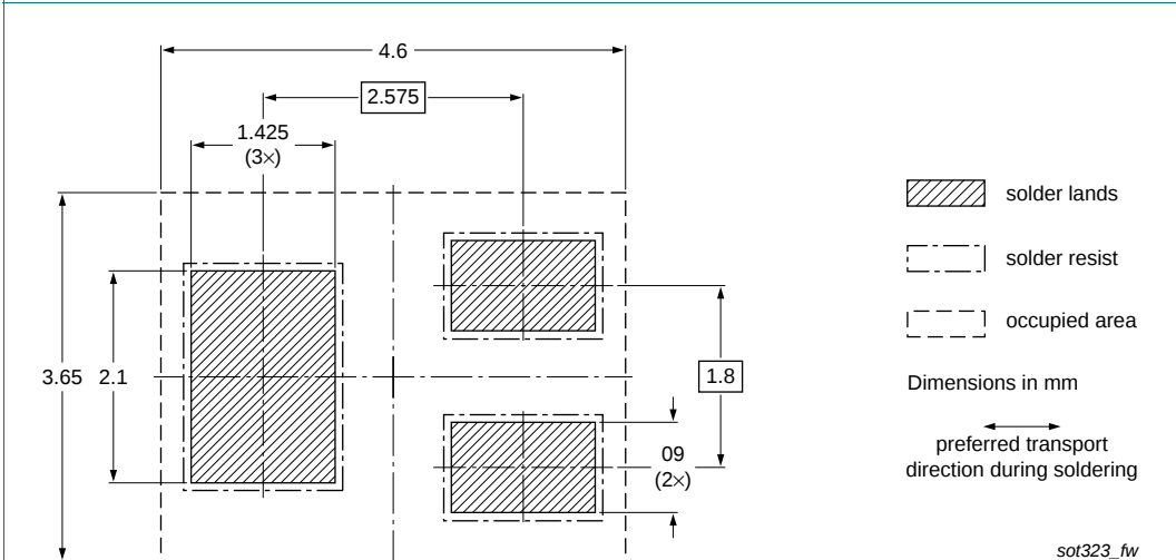
Fig 21. Wave soldering footprint PDTC124EU (SOT323/SC-70)
