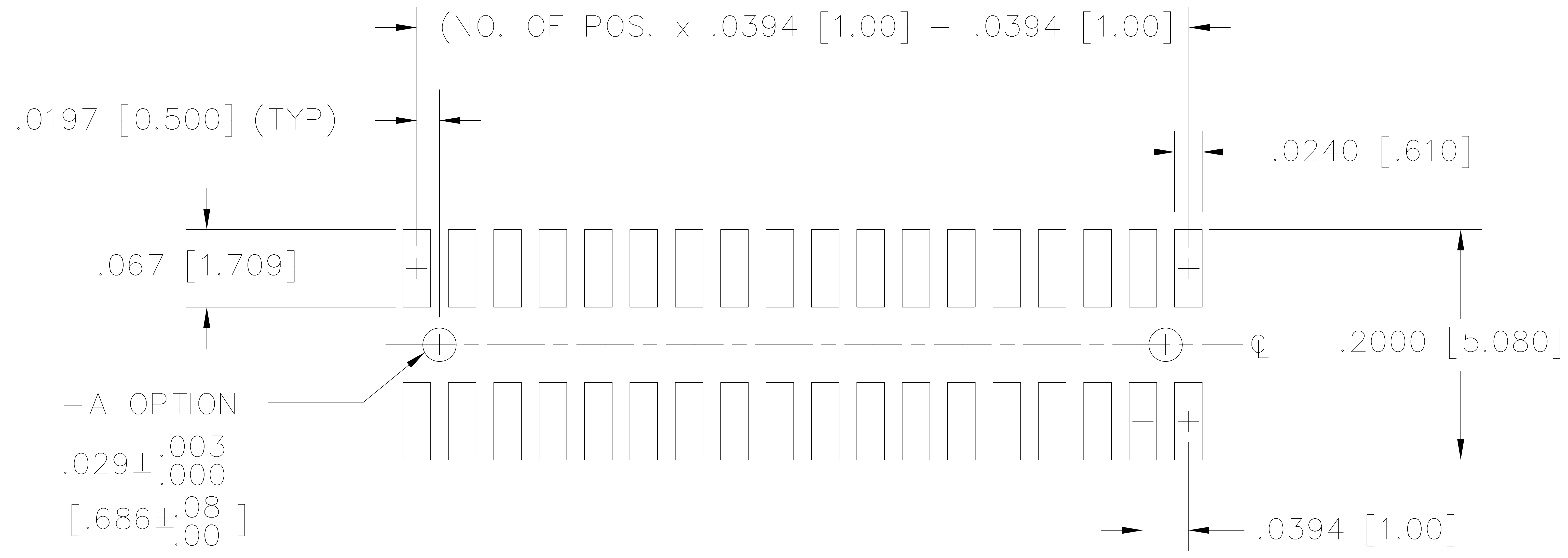
SURFACE MOUNT NON-PASS THRU ENTRY
