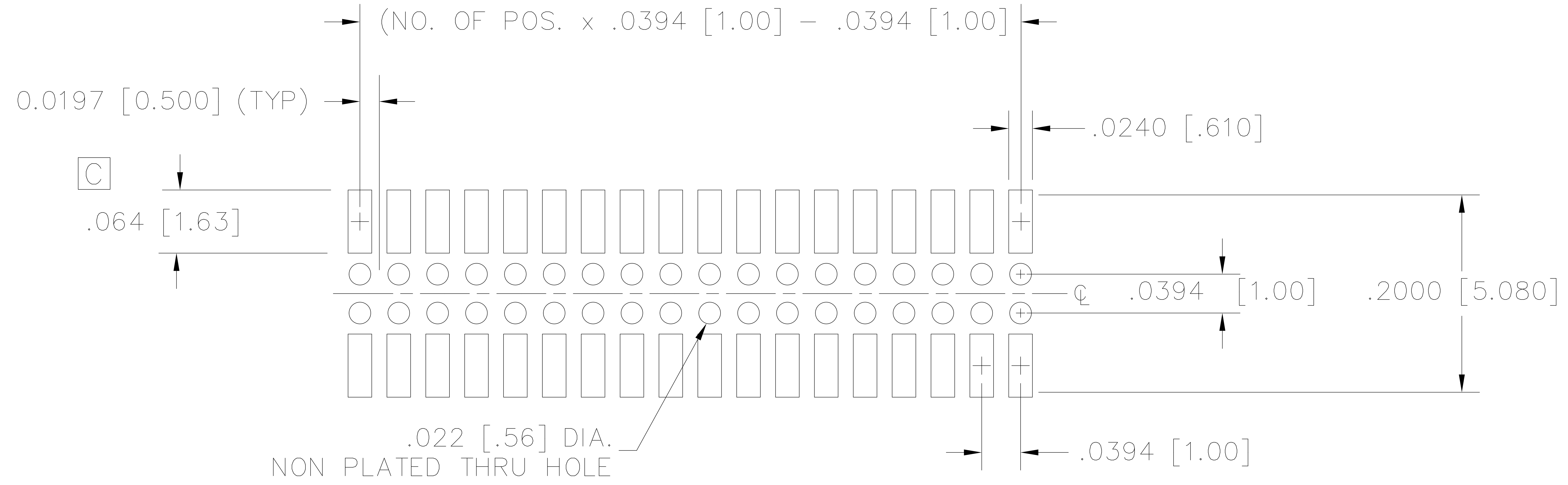
SURFACE MOUNT PASS THRU ENTRY
