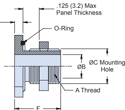
Bulkhead Adapters 710-100/101/372
