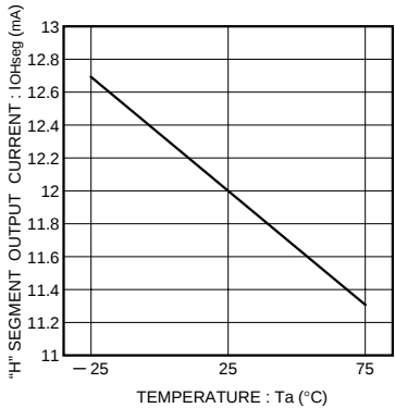
Fig.8 "H" segment output current temperature characteristics
