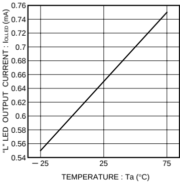
Fig.9 "L" LED output current temperature characteristics
