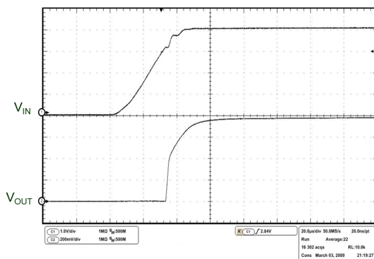
Figure 28. Start-up transient
