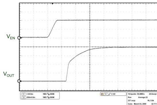
Figure 29. Enable transient
