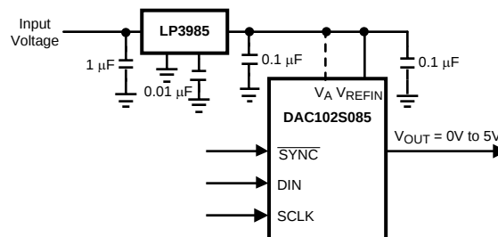
Figure 35. Using the LP3985 regulator
