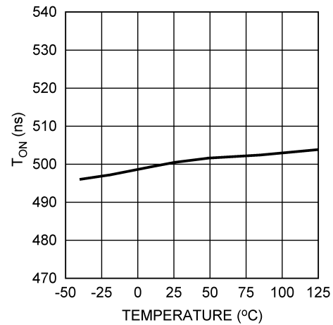
Figure 4. T_{ON} vs Temperature (LM1771S)
