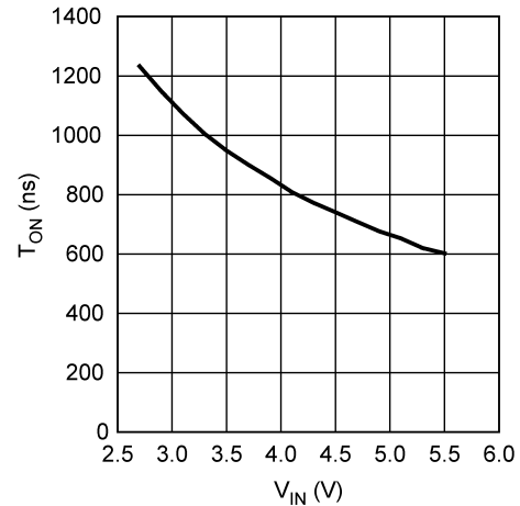
Figure 2. T_{ON} vs V_{IN} (LM1771T)
